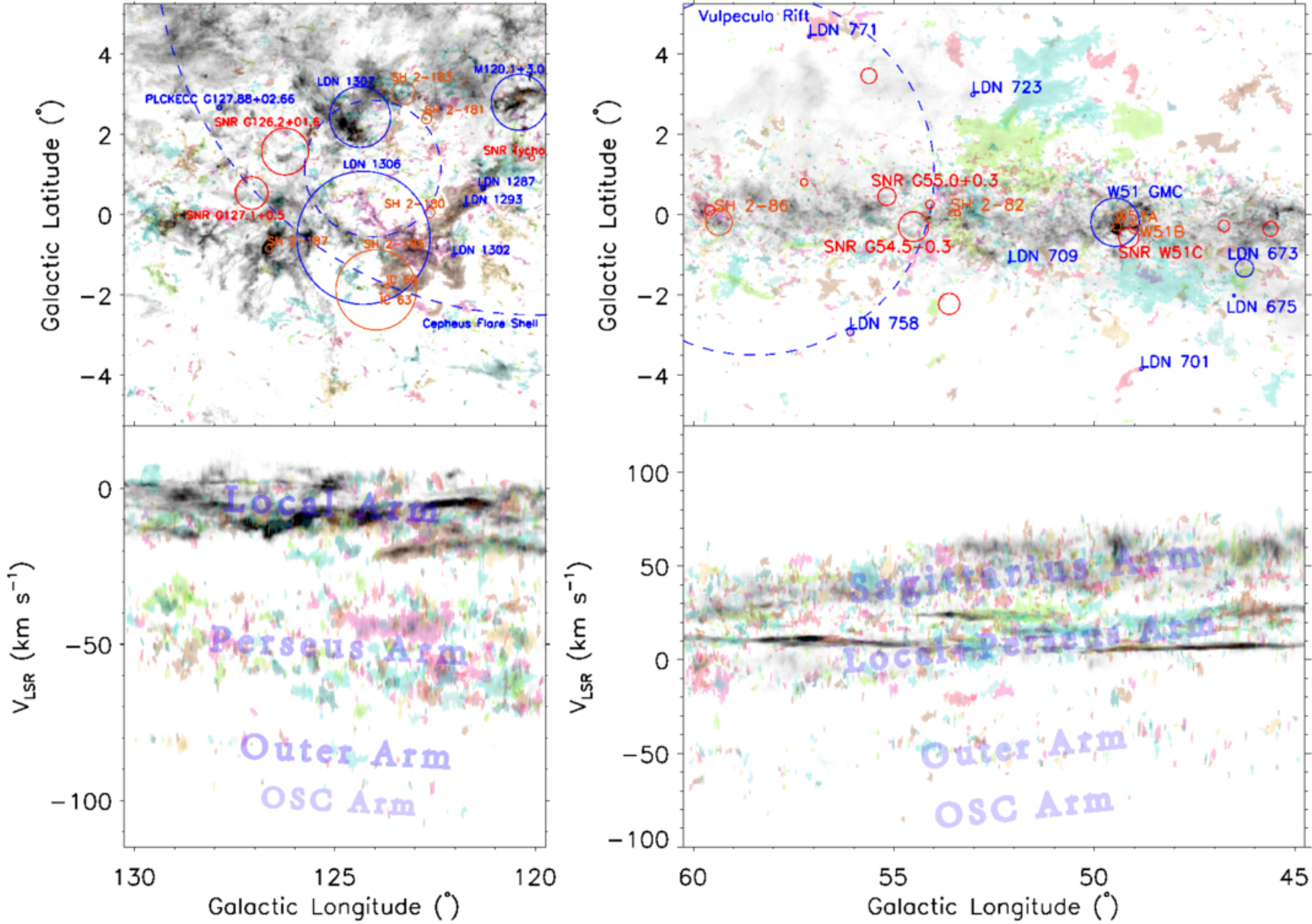
Figure 2. from Xin Zhou et al 2026 Astrophys. J. Suppl. 285 doi:10.3847/1538-4365/ae8155 https://dx.doi.org/10.3847/1538-4365/ae8155 © 2026. The Author(s). Published by the American Astronomical Society.
