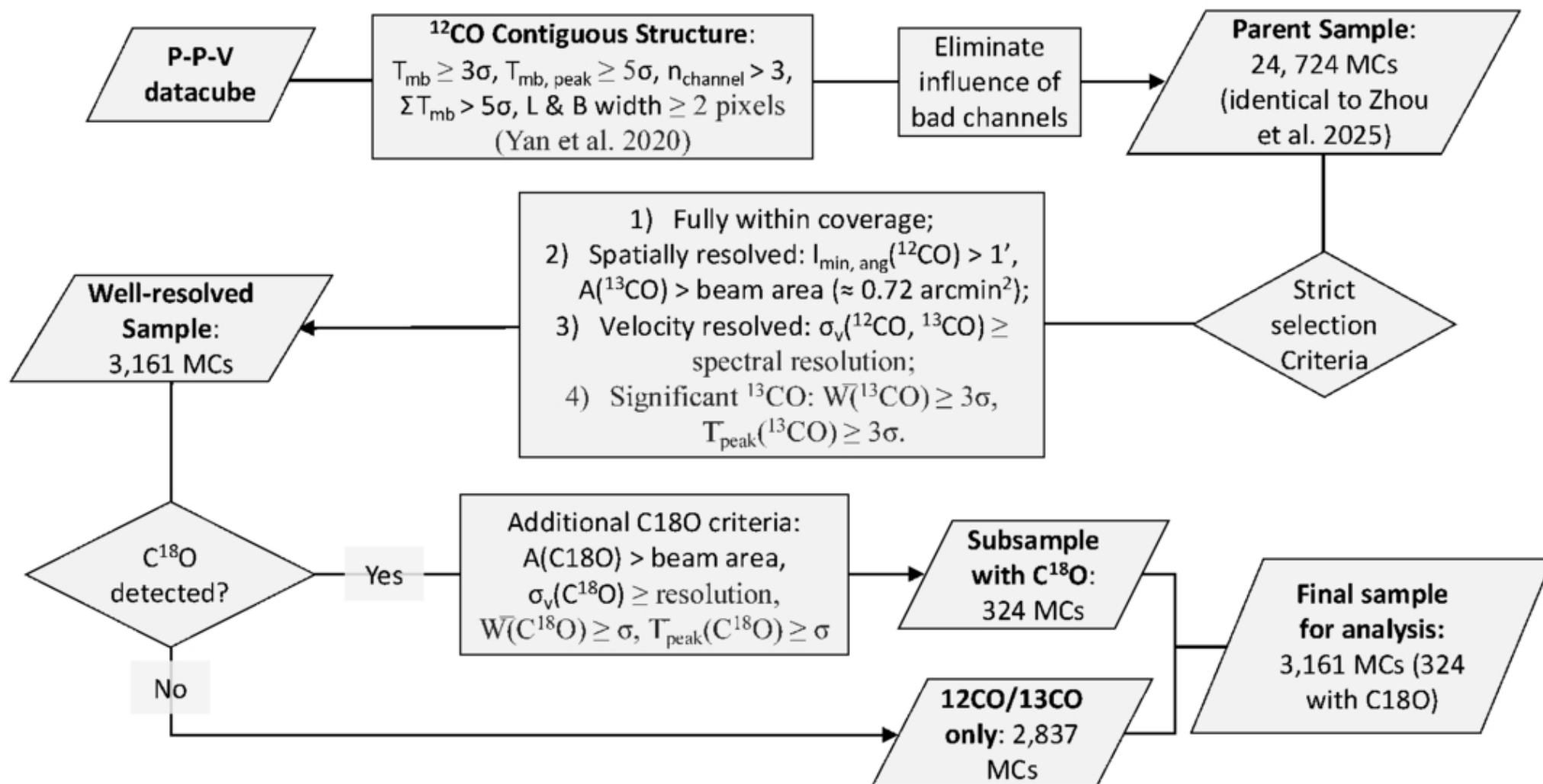
Figure 1. from Xin Zhou et al 2026 Astrophys. J. Suppl. 285 doi:10.3847/1538-4365/ae8155 https://dx.doi.org/10.3847/1538-4365/ae8155 © 2026. The Author(s). Published by the American Astronomical Society.
