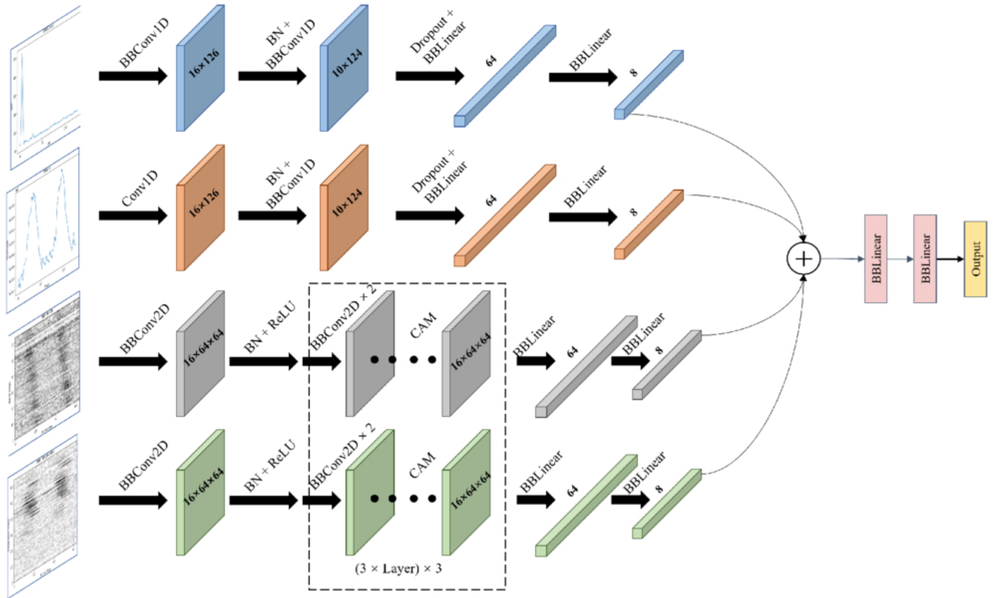
Figure 2. from Yi Liu et al 2026 Astrophys. J. Suppl. 285 doi:10.3847/1538-4365/ae809c https://dx.doi.org/10.3847/1538-4365/ae809c © 2026. The Author(s). Published by the American Astronomical Society.
