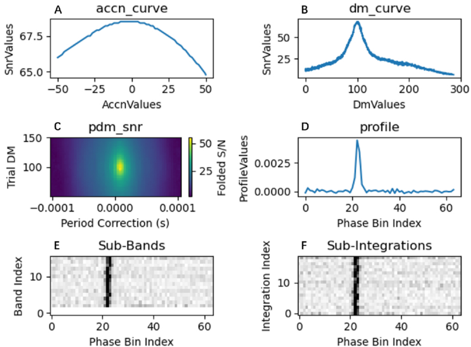
Figure 1. from Yi Liu et al 2026 Astrophys. J. Suppl. 285 doi:10.3847/1538-4365/ae809c https://dx.doi.org/10.3847/1538-4365/ae809c © 2026. The Author(s). Published by the American Astronomical Society.
