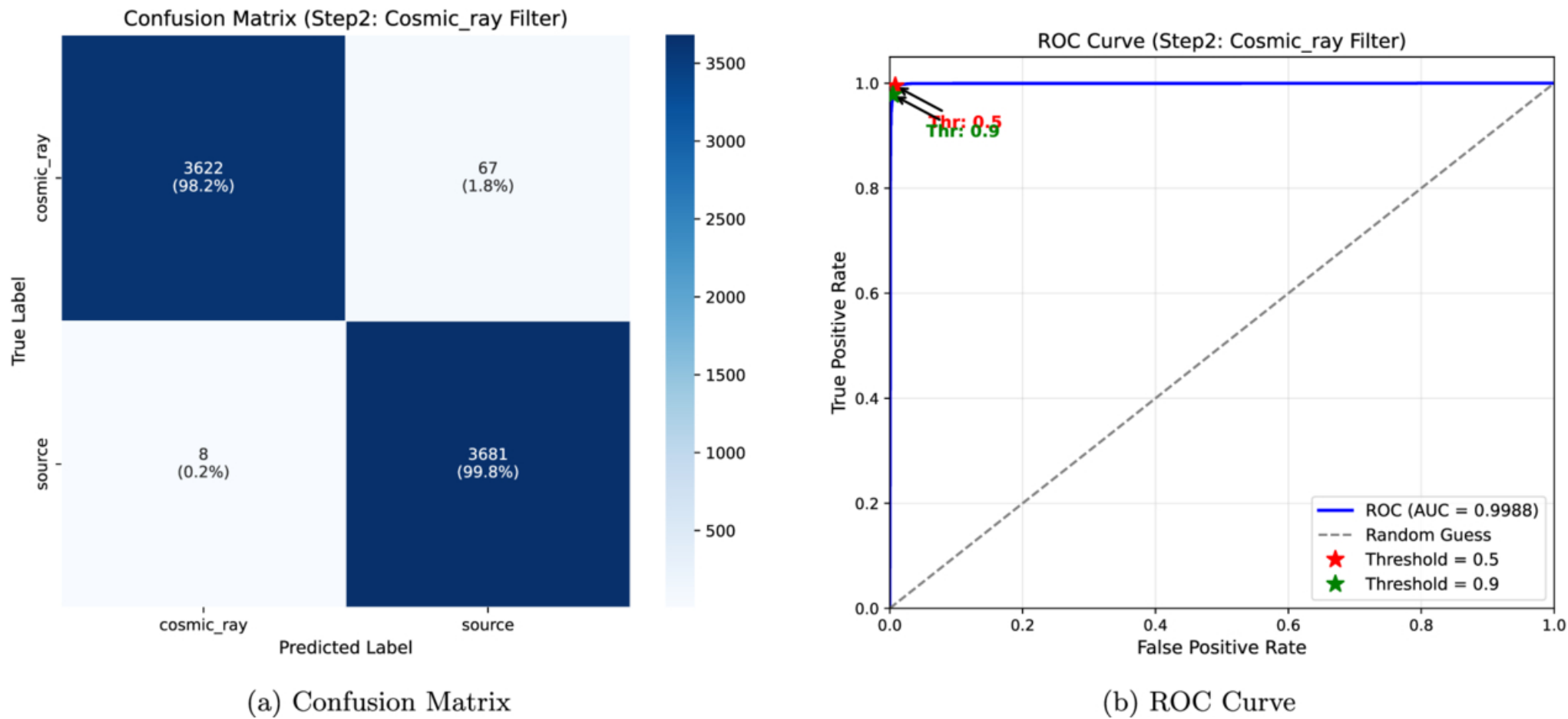
Figure 9. from Lang Chen et al 2026 Astrophys. J. Suppl. 285 doi:10.3847/1538-4365/ae7e7c https://dx.doi.org/10.3847/1538-4365/ae7e7c © 2026. The Author(s). Published by the American Astronomical Society.
