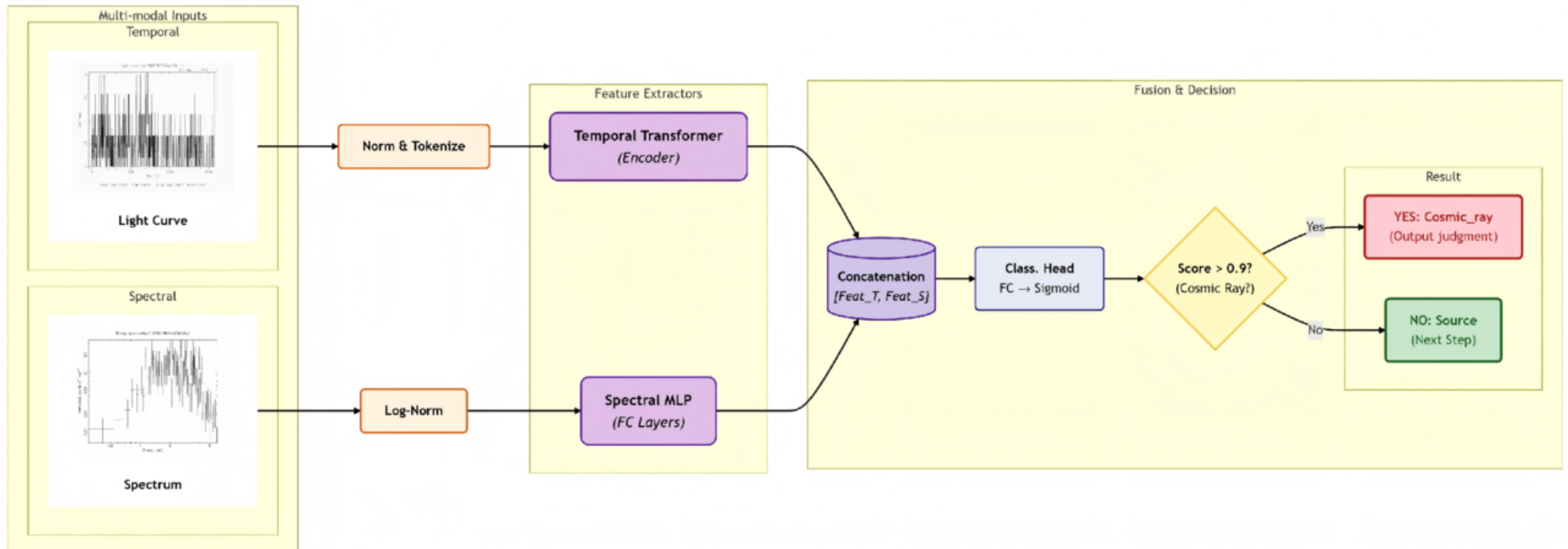
Figure 6. from Lang Chen et al 2026 Astrophys. J. Suppl. 285 doi:10.3847/1538-4365/ae7e7c https://dx.doi.org/10.3847/1538-4365/ae7e7c © 2026. The Author(s). Published by the American Astronomical Society.
