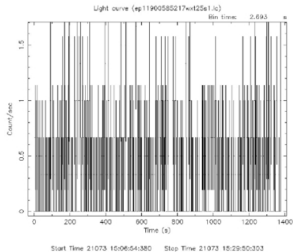
(a) Arm: Light Curve
