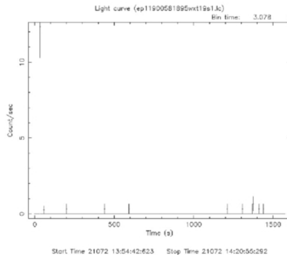
(b) Cosmic Ray: Light Curve
