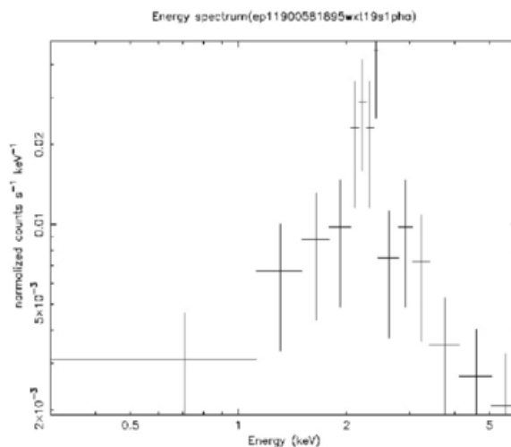
(e) Cosmic Ray: Spectrum
