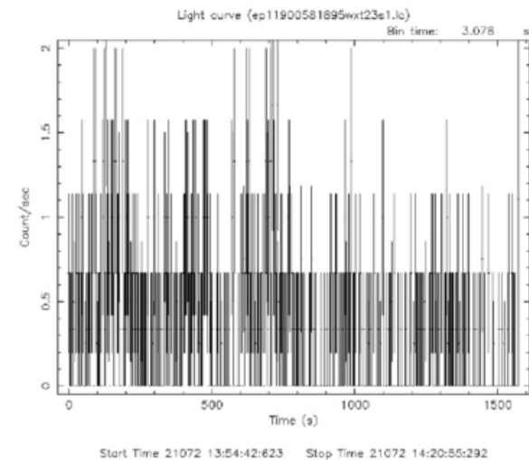
(c) Source: Light Curve
