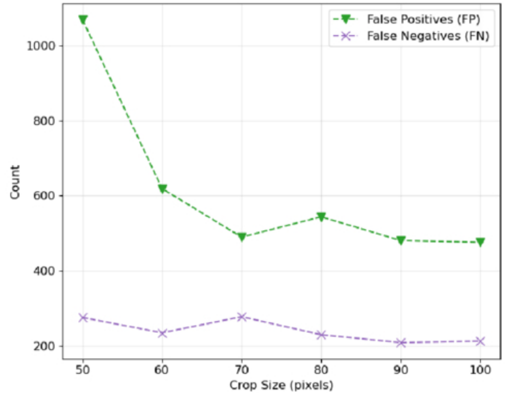
(b) Error Count Trend vs. Crop Size
