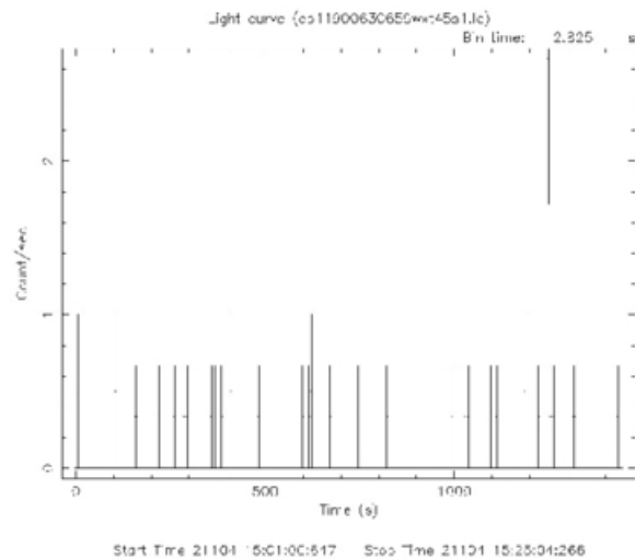
(a) Case 1: Light curve
