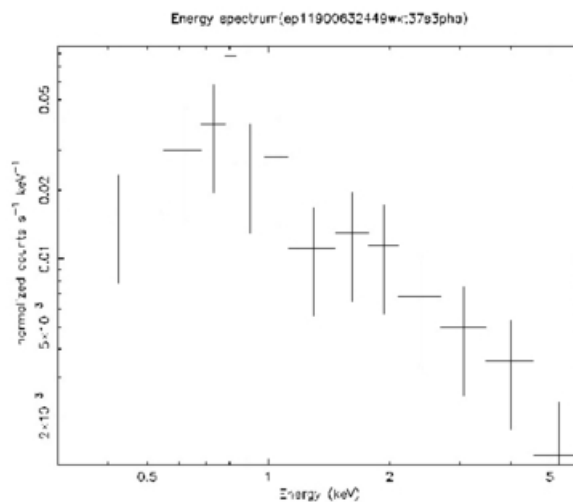
(e) Case 2: PI spectrum
