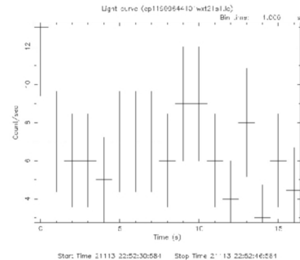
(c) ep11900644101wxt21s1: Light curve
