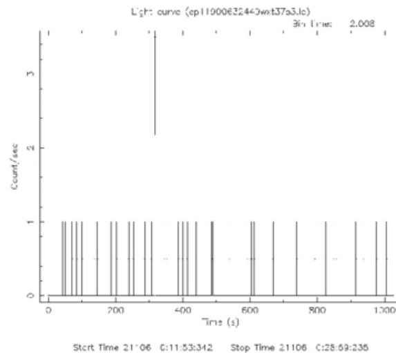
(b) Case 2: Light curve
