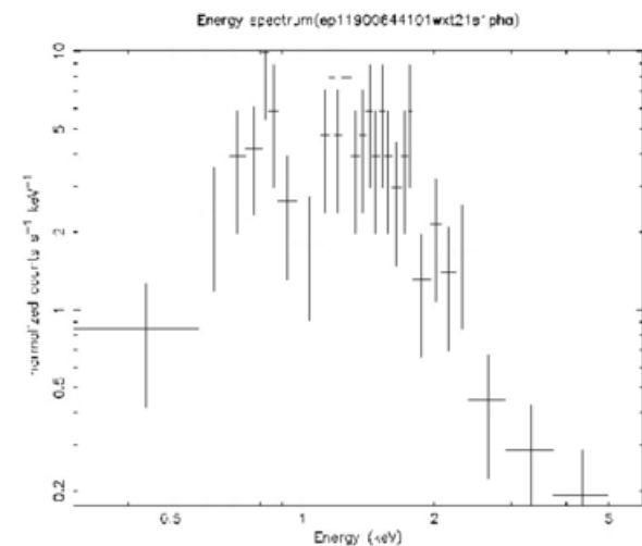
(f) ep11900644101wxt21s1: PI spectrum
