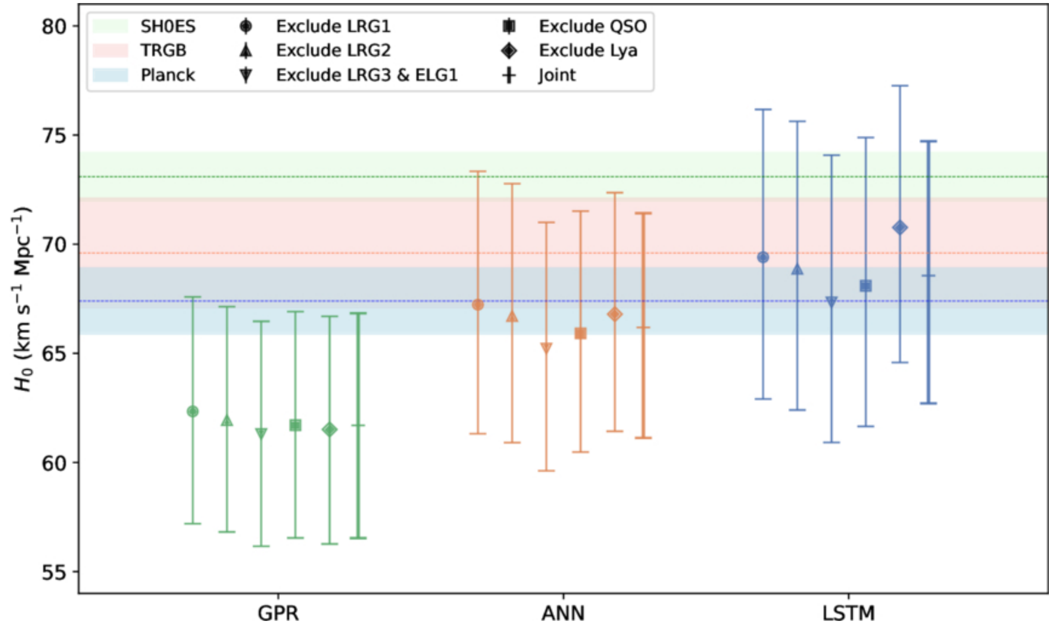
Figure 9. from Chenfa Zheng et al 2026 Astrophys. J. Suppl. 285 doi:10.3847/1538-4365/ae7d1a https://dx.doi.org/10.3847/1538-4365/ae7d1a © 2026. The Author(s). Published by the American Astronomical Society.
