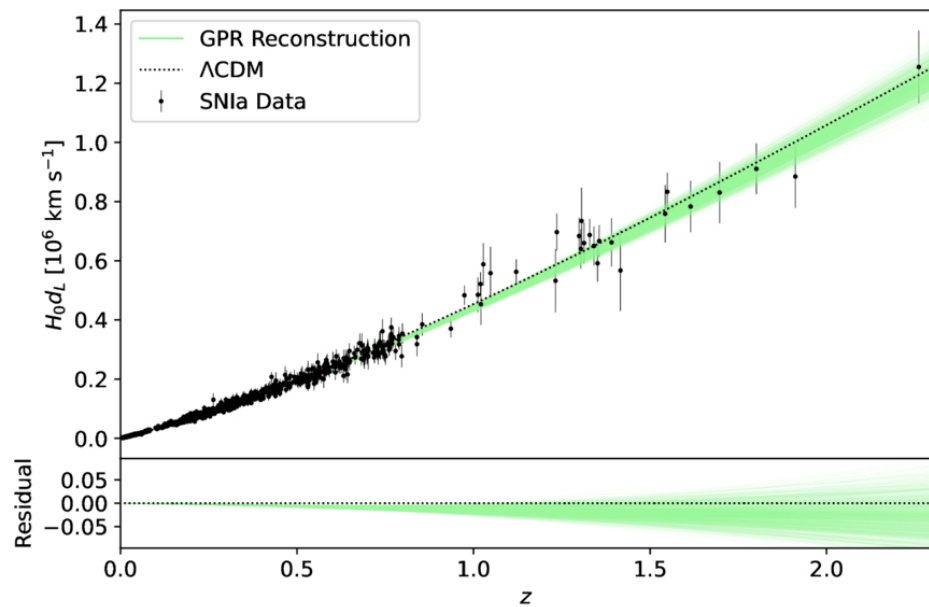
Figure 7. from Chenfa Zheng et al 2026 Astrophys. J. Suppl. 285 doi:10.3847/1538-4365/ae7d1a https://dx.doi.org/10.3847/1538-4365/ae7d1a © 2026. The Author(s). Published by the American Astronomical Society.
