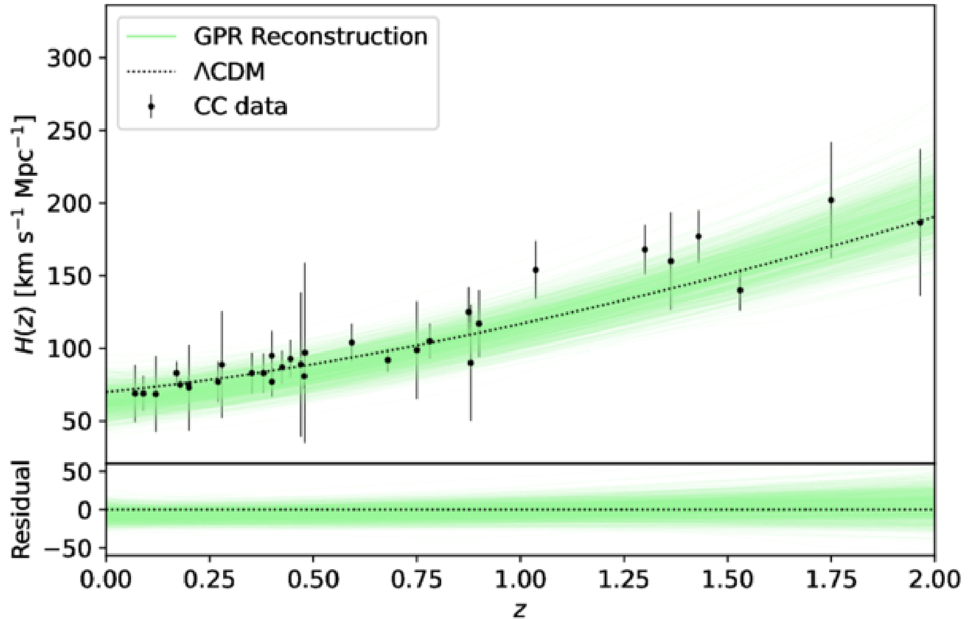
Figure 5. from Chenfa Zheng et al 2026 Astrophys. J. Suppl. 285 doi:10.3847/1538-4365/ae7d1a https://dx.doi.org/10.3847/1538-4365/ae7d1a © 2026. The Author(s). Published by the American Astronomical Society.
