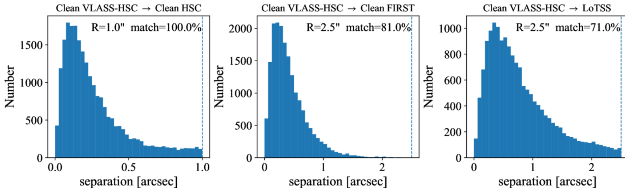
Figure 8. from Hisakazu Uchiyama et al 2026 Astrophys. J. Suppl. 285 doi:10.3847/1538-4365/ae7bff https://dx.doi.org/10.3847/1538-4365/ae7bff © 2026. The Author(s). Published by the American Astronomical Society.
