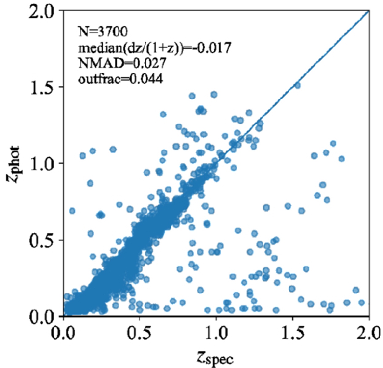
Figure 5. from Hisakazu Uchiyama et al 2026 Astrophys. J. Suppl. 285 doi:10.3847/1538-4365/ae7bff https://dx.doi.org/10.3847/1538-4365/ae7bff © 2026. The Author(s). Published by the American Astronomical Society.
