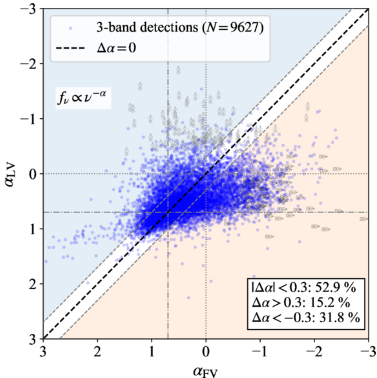
Figure 3. from Hisakazu Uchiyama et al 2026 Astrophys. J. Suppl. 285 doi:10.3847/1538-4365/ae7bff https://dx.doi.org/10.3847/1538-4365/ae7bff © 2026. The Author(s). Published by the American Astronomical Society.
