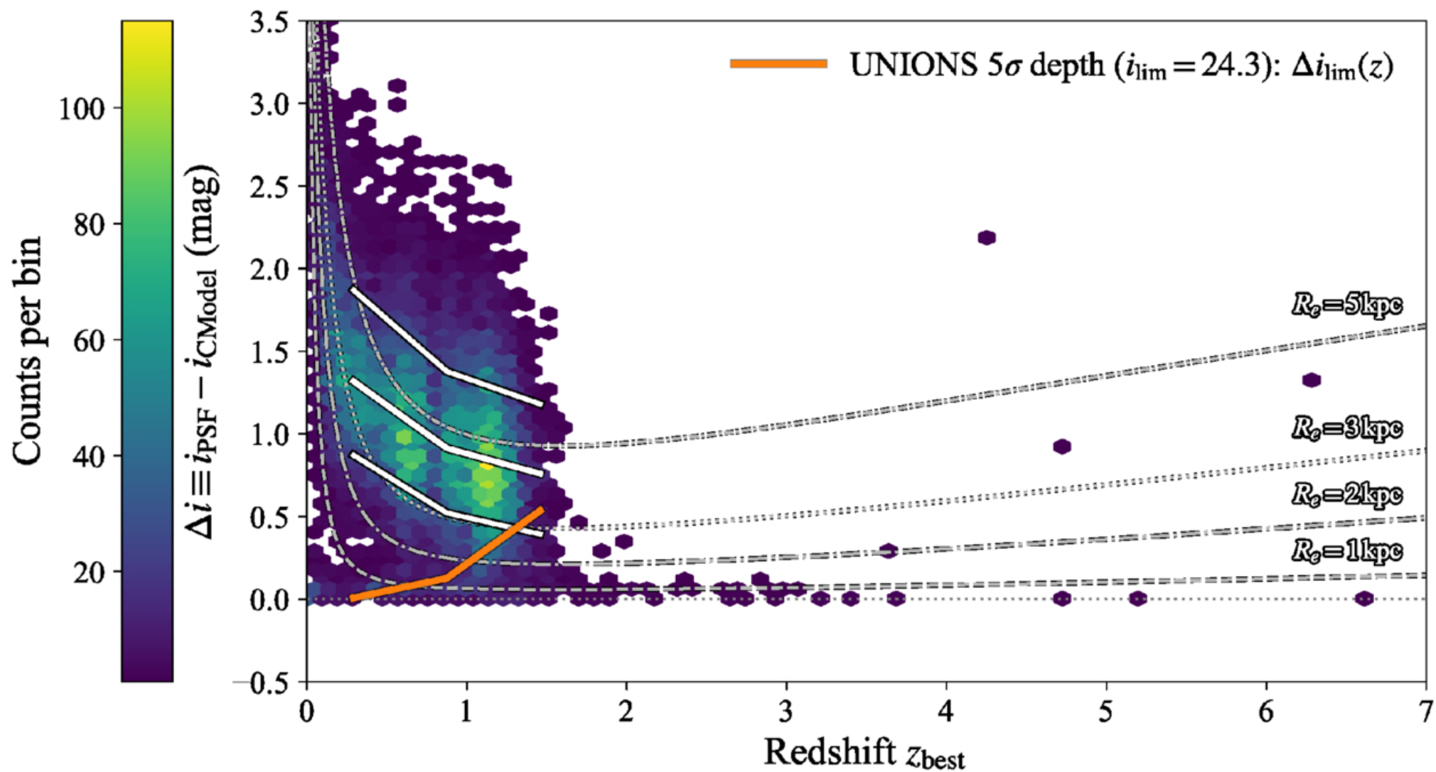
Figure 14. from Hisakazu Uchiyama et al 2026 Astrophys. J. Suppl. 285 doi:10.3847/1538-4365/ae7bff https://dx.doi.org/10.3847/1538-4365/ae7bff © 2026. The Author(s). Published by the American Astronomical Society.
