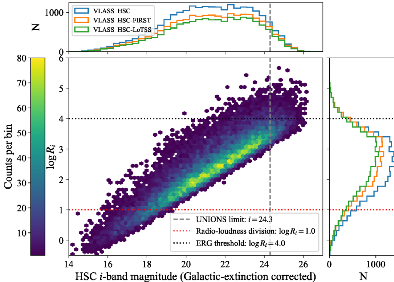
Figure 11. from Hisakazu Uchiyama et al 2026 Astrophys. J. Suppl. 285 doi:10.3847/1538-4365/ae7bff https://dx.doi.org/10.3847/1538-4365/ae7bff © 2026. The Author(s). Published by the American Astronomical Society.
