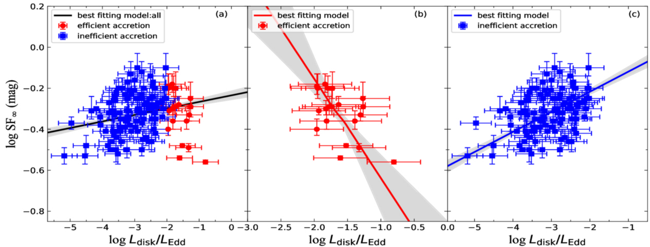
Figure 4. from Yongyun Chen et al 2026 Astrophys. J. Suppl. 285 doi:10.3847/1538-4365/ae7a52 https://dx.doi.org/10.3847/1538-4365/ae7a52 © 2026. The Author(s). Published by the American Astronomical Society.
