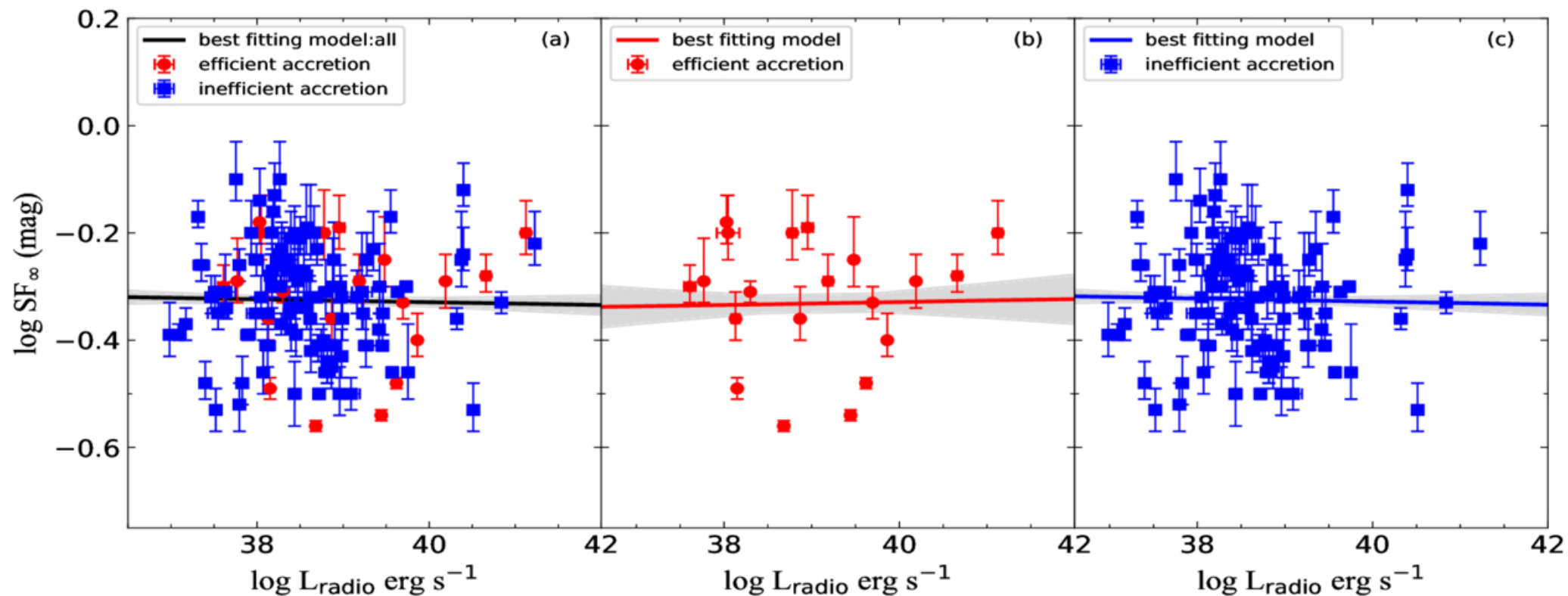
Figure 3. from Yongyun Chen et al 2026 Astrophys. J. Suppl. 285 doi:10.3847/1538-4365/ae7a52 https://dx.doi.org/10.3847/1538-4365/ae7a52 © 2026. The Author(s). Published by the American Astronomical Society.
