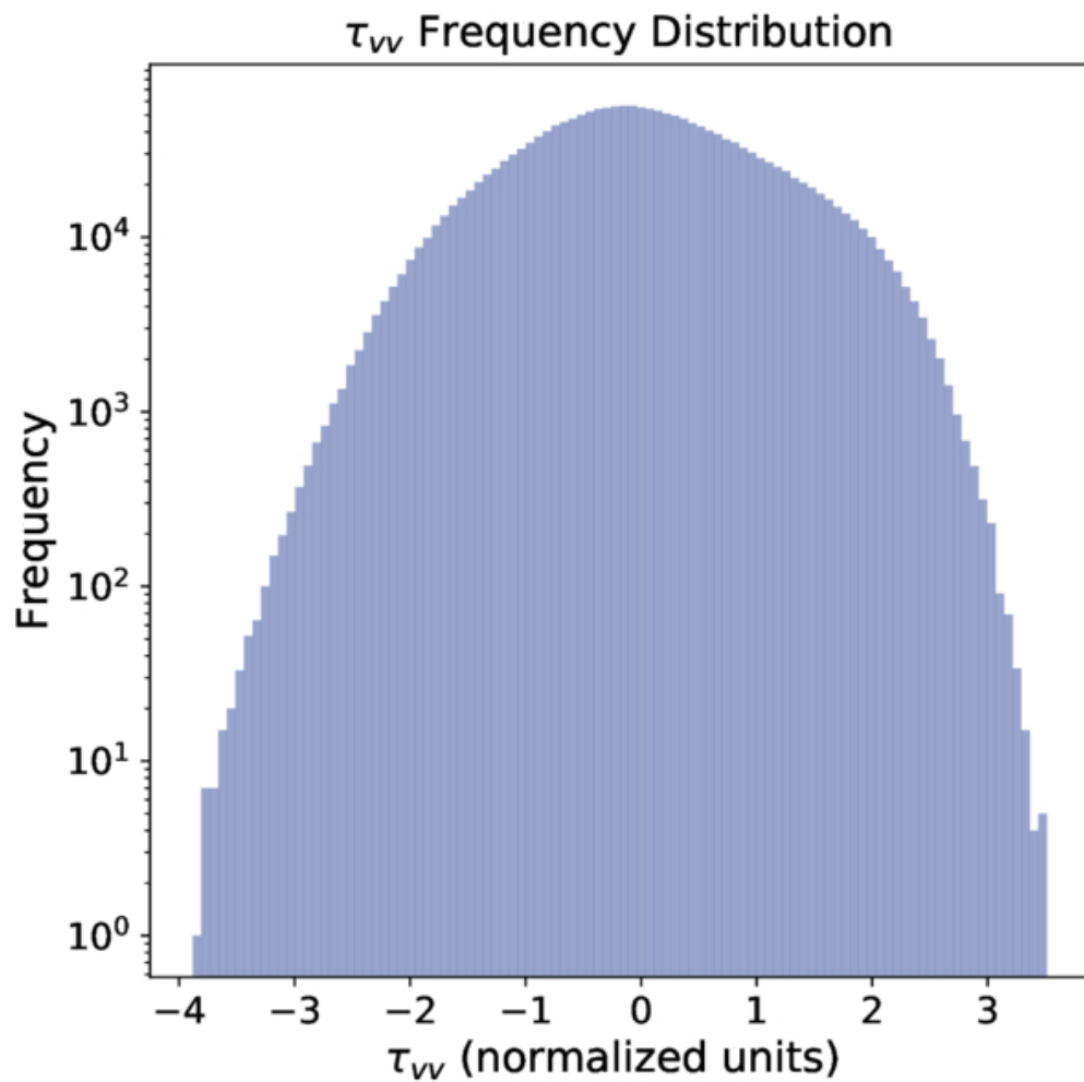
Figure 2. from Rimsha Hameed Syeda et al 2026 Astrophys. J. Suppl. 285 doi:10.3847/1538-4365/ae78cf https://dx.doi.org/10.3847/1538-4365/ae78cf © 2026. The Author(s). Published by the American Astronomical Society.
