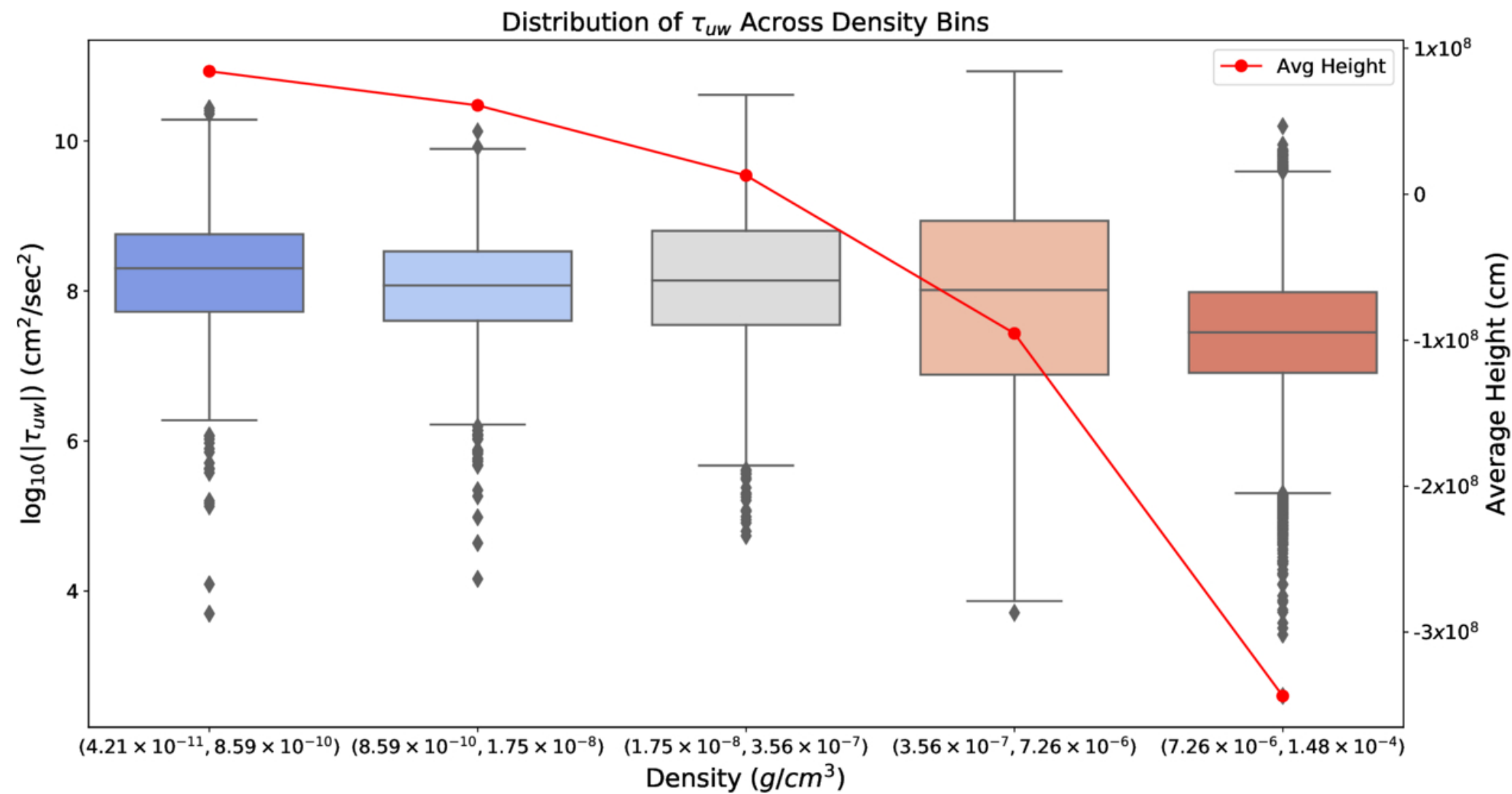
Figure 16. from Rimsha Hameed Syeda et al 2026 Astrophys. J. Suppl. 285 doi:10.3847/1538-4365/ae78cf https://dx.doi.org/10.3847/1538-4365/ae78cf © 2026. The Author(s). Published by the American Astronomical Society.
