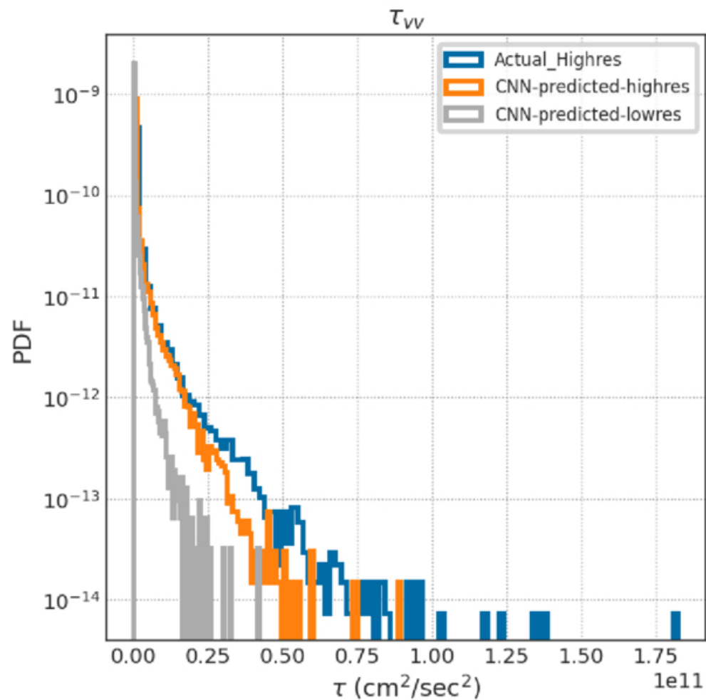
Figure 13. from Rimsha Hameed Syeda et al 2026 Astrophys. J. Suppl. 285 doi:10.3847/1538-4365/ae78cf https://dx.doi.org/10.3847/1538-4365/ae78cf © 2026. The Author(s). Published by the American Astronomical Society.
