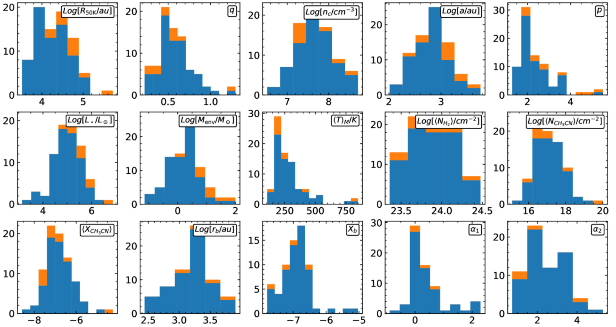
Figure 5. from Dezhao Meng et al 2026 Astrophys. J. Suppl. 285 doi:10.3847/1538-4365/ae77e7 https://dx.doi.org/10.3847/1538-4365/ae77e7 © 2026. The Author(s). Published by the American Astronomical Society.
