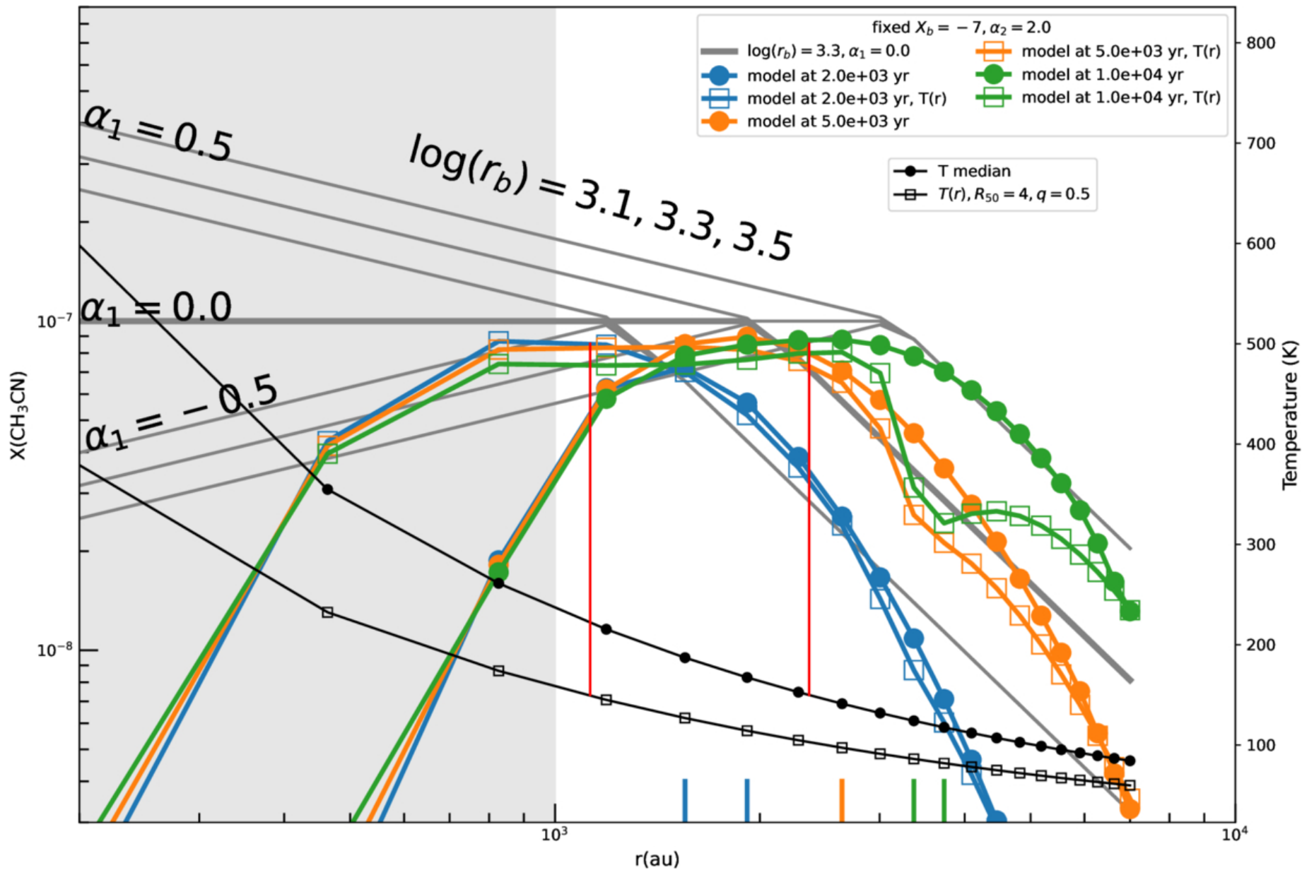
Figure C1. from Dezhao Meng et al 2026 Astrophys. J. Suppl. 285 doi:10.3847/1538-4365/ae77e7 https://dx.doi.org/10.3847/1538-4365/ae77e7 © 2026. The Author(s). Published by the American Astronomical Society.
