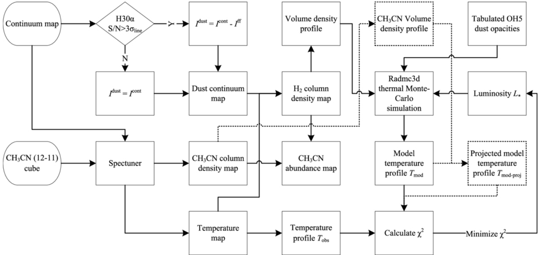
Figure 1. from Dezhao Meng et al 2026 Astrophys. J. Suppl. 285 doi:10.3847/1538-4365/ae77e7 https://dx.doi.org/10.3847/1538-4365/ae77e7 © 2026. The Author(s). Published by the American Astronomical Society.
