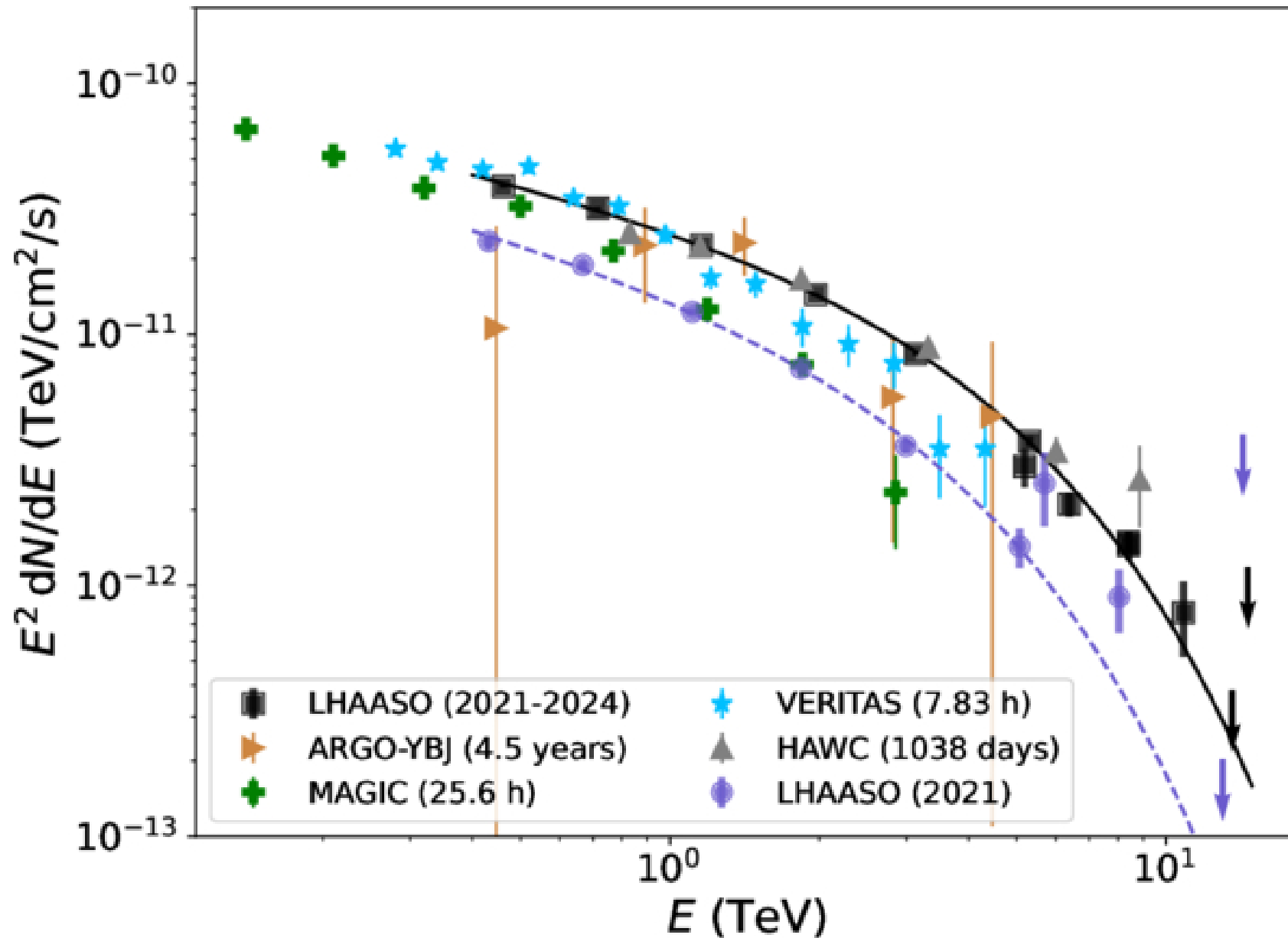
Figure 9. from Zhen Cao et al 2026 Astrophys. J. Suppl. 285 doi:10.3847/1538-4365/ae76cc https://dx.doi.org/10.3847/1538-4365/ae76cc © 2026. The Author(s). Published by the American Astronomical Society.
