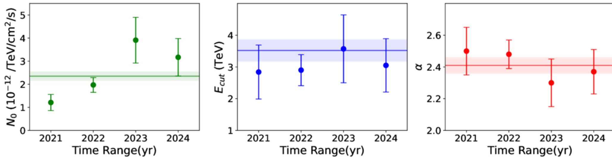
Figure 8. from Zhen Cao et al 2026 Astrophys. J. Suppl. 285 doi:10.3847/1538-4365/ae76cc https://dx.doi.org/10.3847/1538-4365/ae76cc © 2026. The Author(s). Published by the American Astronomical Society.
