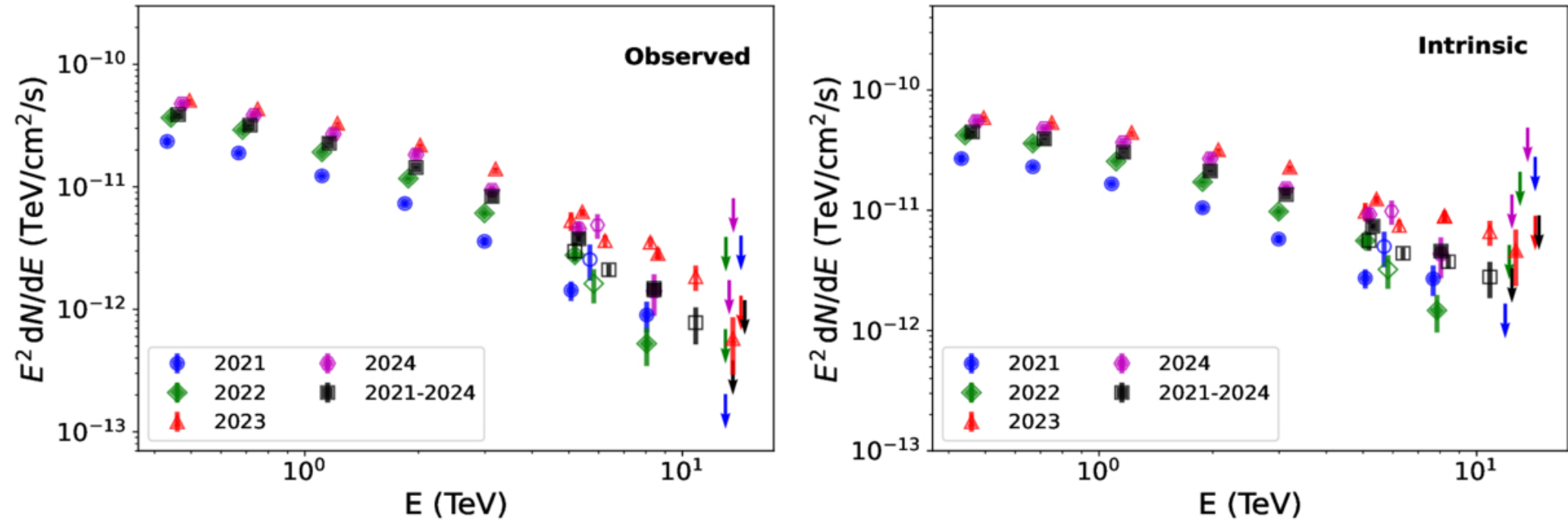
Figure 7. from Zhen Cao et al 2026 Astrophys. J. Suppl. 285 doi:10.3847/1538-4365/ae76cc https://dx.doi.org/10.3847/1538-4365/ae76cc © 2026. The Author(s). Published by the American Astronomical Society.
