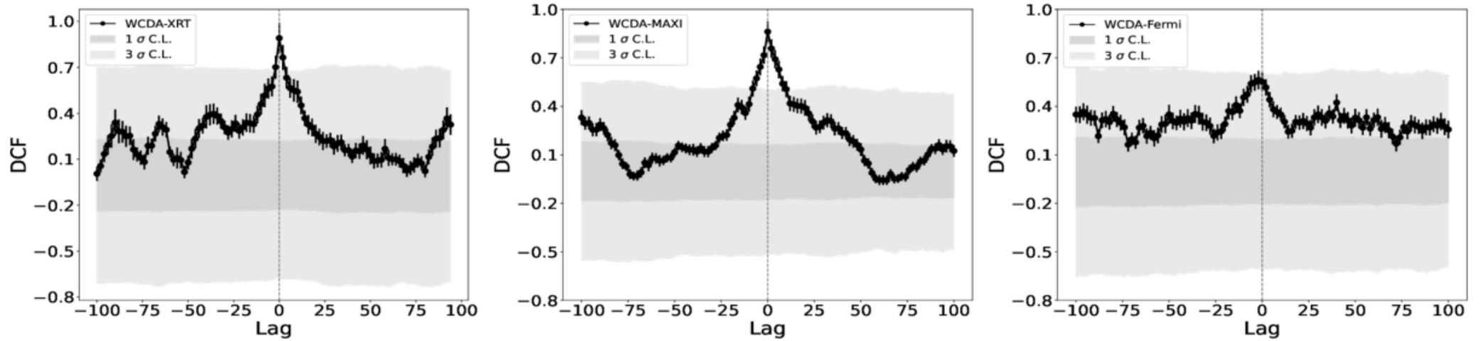
Figure 6. from Zhen Cao et al 2026 Astrophys. J. Suppl. 285 doi:10.3847/1538-4365/ae76cc https://dx.doi.org/10.3847/1538-4365/ae76cc © 2026. The Author(s). Published by the American Astronomical Society.
