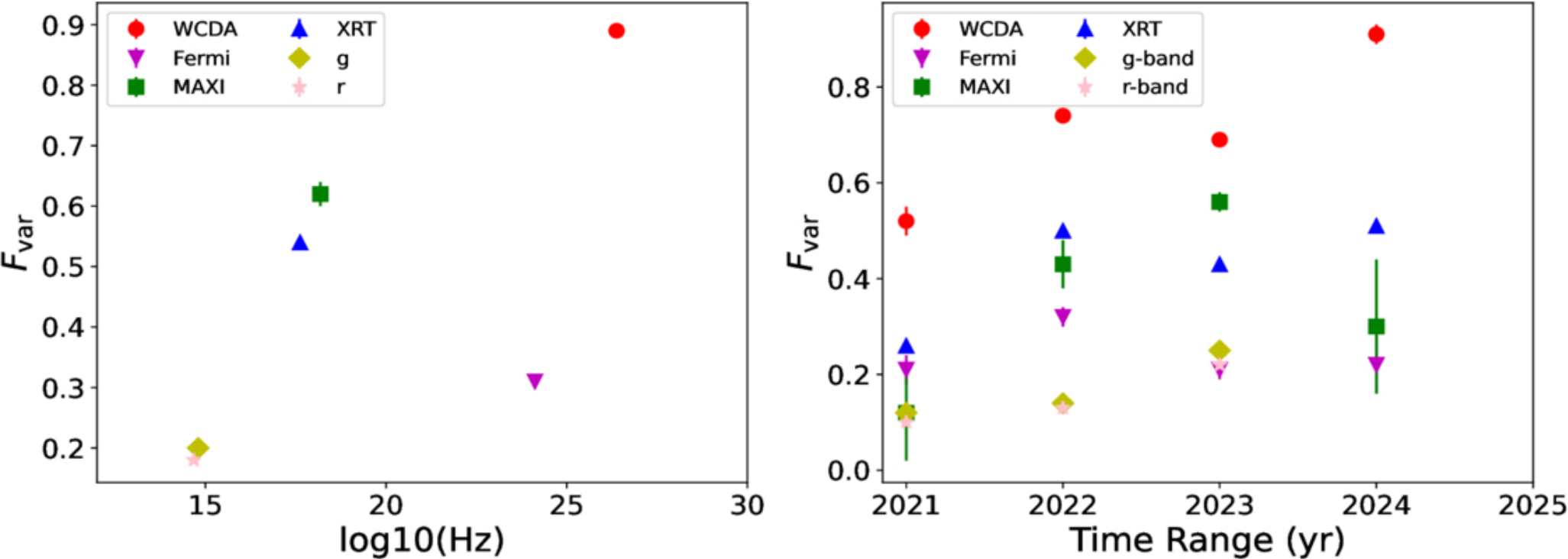
Figure 5. from Zhen Cao et al 2026 Astrophys. J. Suppl. 285 doi:10.3847/1538-4365/ae76cc https://dx.doi.org/10.3847/1538-4365/ae76cc © 2026. The Author(s). Published by the American Astronomical Society.
