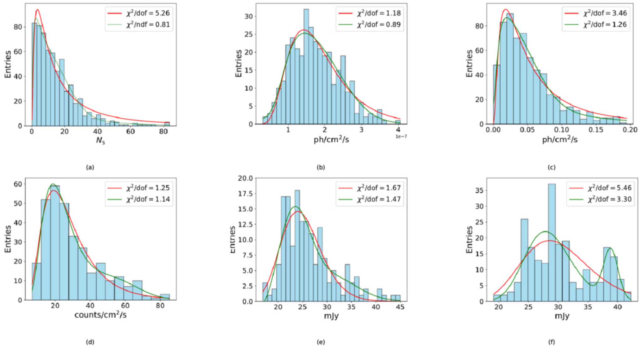
Figure 4. from Zhen Cao et al 2026 Astrophys. J. Suppl. 285 doi:10.3847/1538-4365/ae76cc https://dx.doi.org/10.3847/1538-4365/ae76cc © 2026. The Author(s). Published by the American Astronomical Society.
