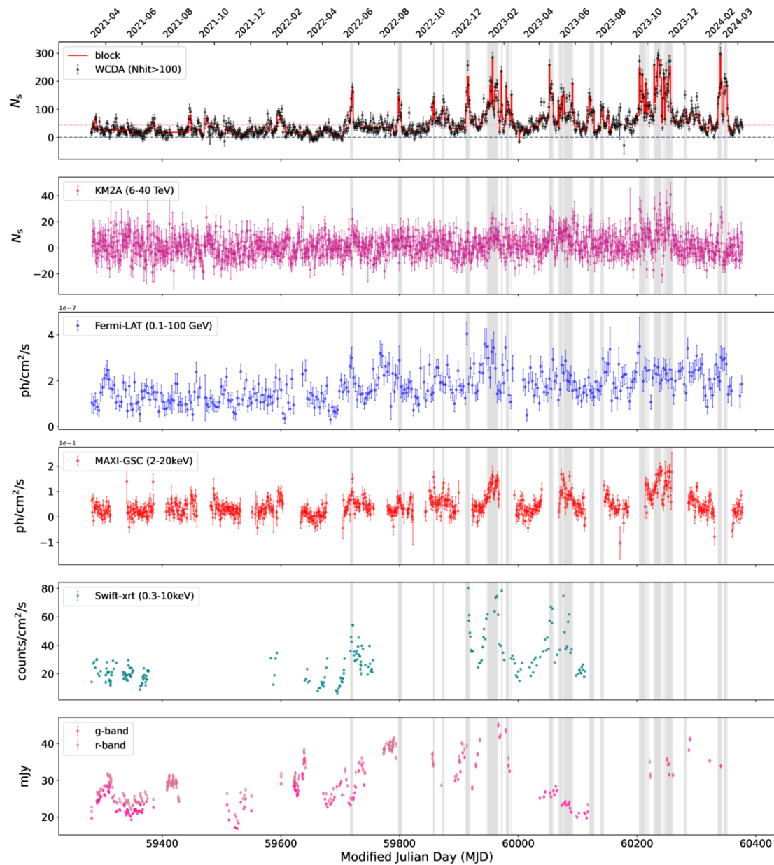
Figure 2. from Zhen Cao et al 2026 Astrophys. J. Suppl. 285 doi:10.3847/1538-4365/ae76cc https://dx.doi.org/10.3847/1538-4365/ae76cc © 2026. The Author(s). Published by the American Astronomical Society.
