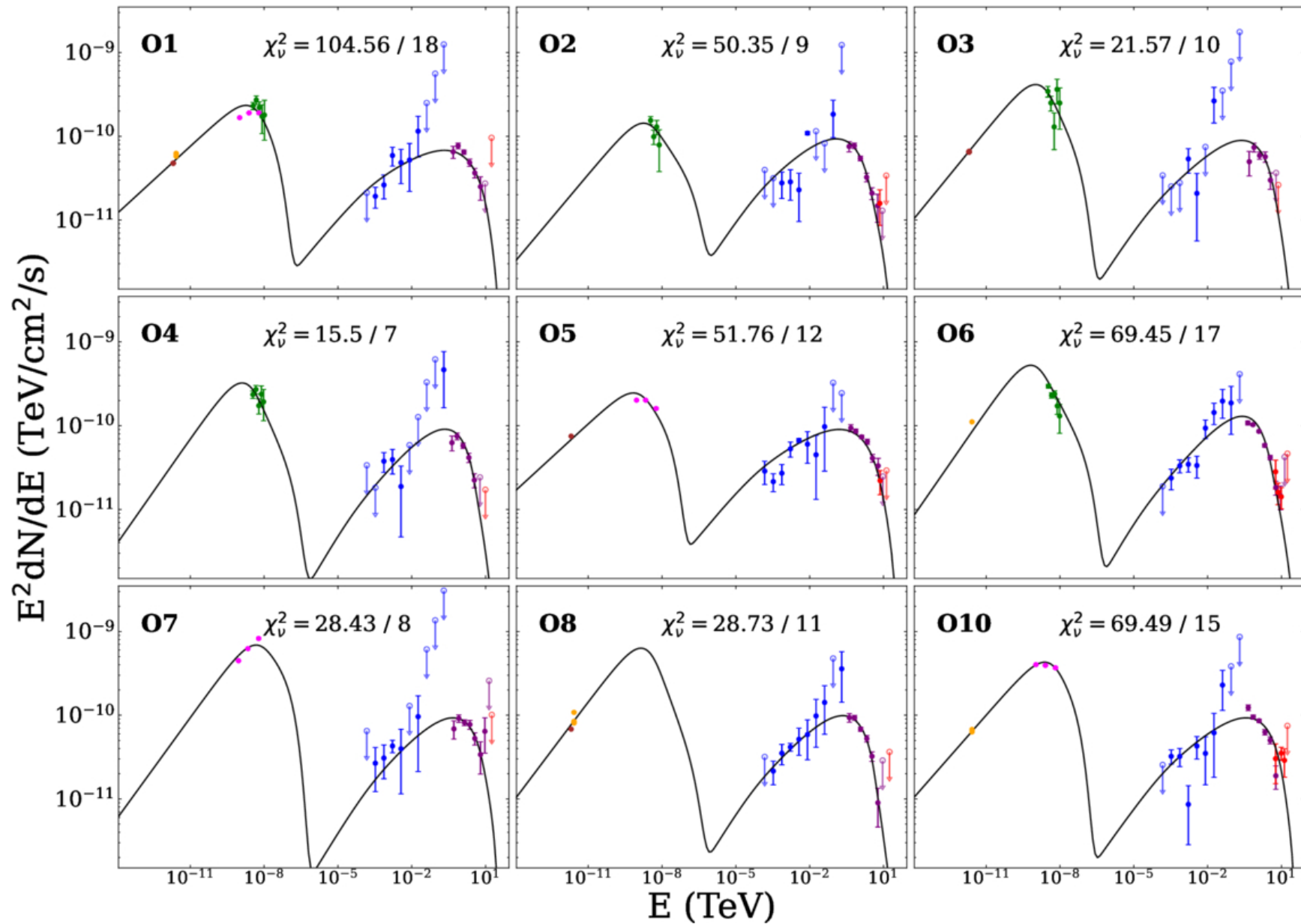
Figure 18. from Zhen Cao et al 2026 Astrophys. J. Suppl. 285 doi:10.3847/1538-4365/ae76cc https://dx.doi.org/10.3847/1538-4365/ae76cc © 2026. The Author(s). Published by the American Astronomical Society.
