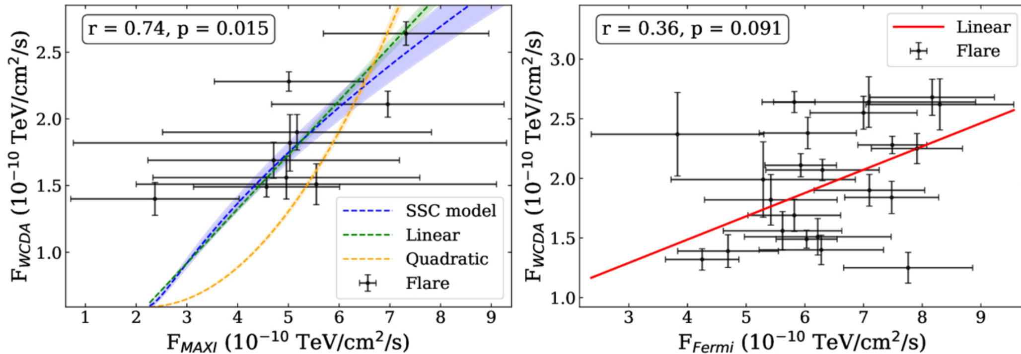
Figure 17. from Zhen Cao et al 2026 Astrophys. J. Suppl. 285 doi:10.3847/1538-4365/ae76cc https://dx.doi.org/10.3847/1538-4365/ae76cc © 2026. The Author(s). Published by the American Astronomical Society.
