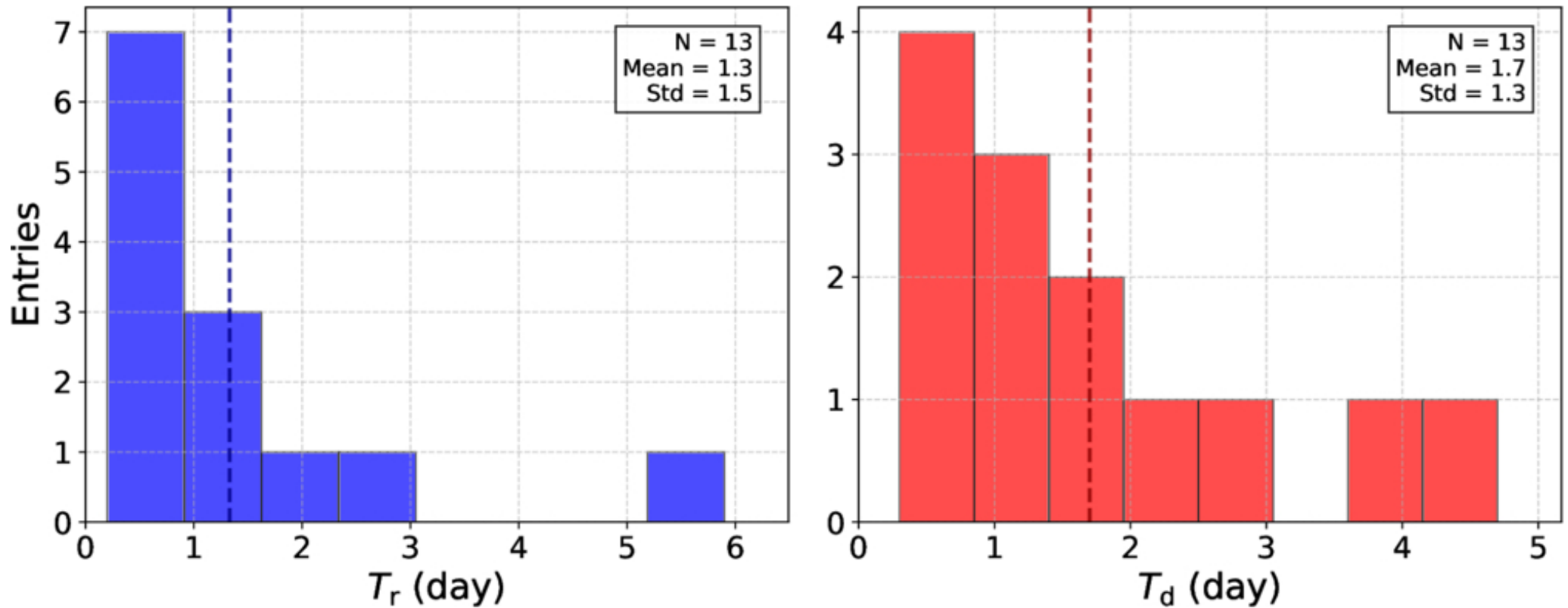
Figure 13. from Zhen Cao et al 2026 Astrophys. J. Suppl. 285 doi:10.3847/1538-4365/ae76cc https://dx.doi.org/10.3847/1538-4365/ae76cc © 2026. The Author(s). Published by the American Astronomical Society.
