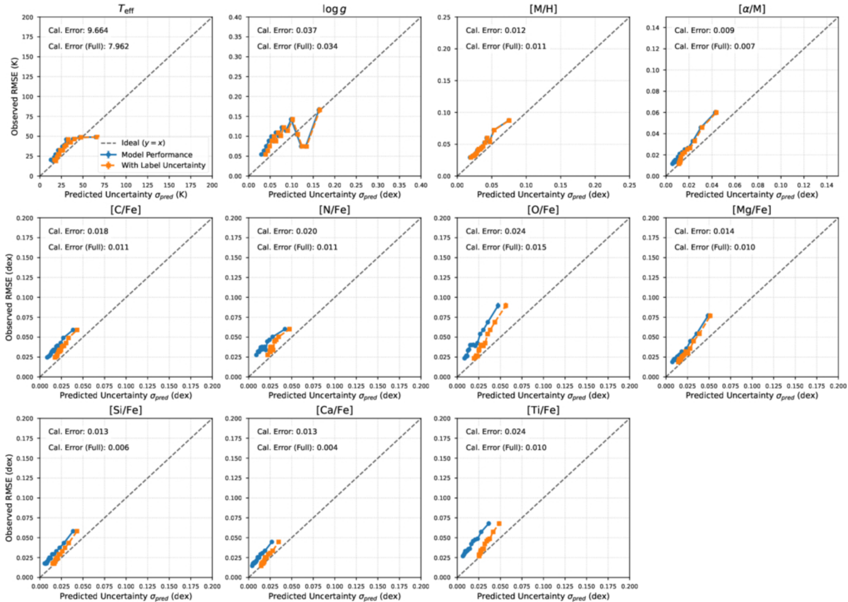
Figure 8. from Jingzhen Sun et al 2026 Astrophys. J. Suppl. 285 doi:10.3847/1538-4365/ae743e https://dx.doi.org/10.3847/1538-4365/ae743e © 2026. The Author(s). Published by the American Astronomical Society.
