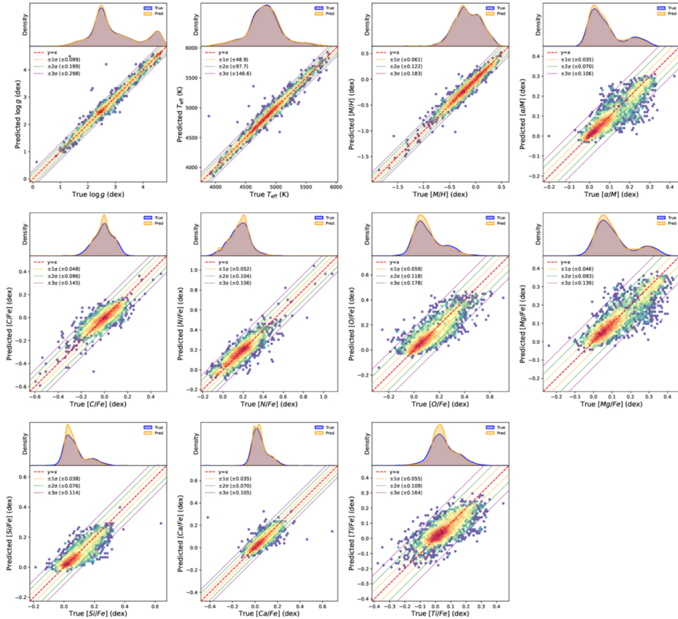
Figure 4. from Jingzhen Sun et al 2026 Astrophys. J. Suppl. 285 doi:10.3847/1538-4365/ae743e https://dx.doi.org/10.3847/1538-4365/ae743e © 2026. The Author(s). Published by the American Astronomical Society.
