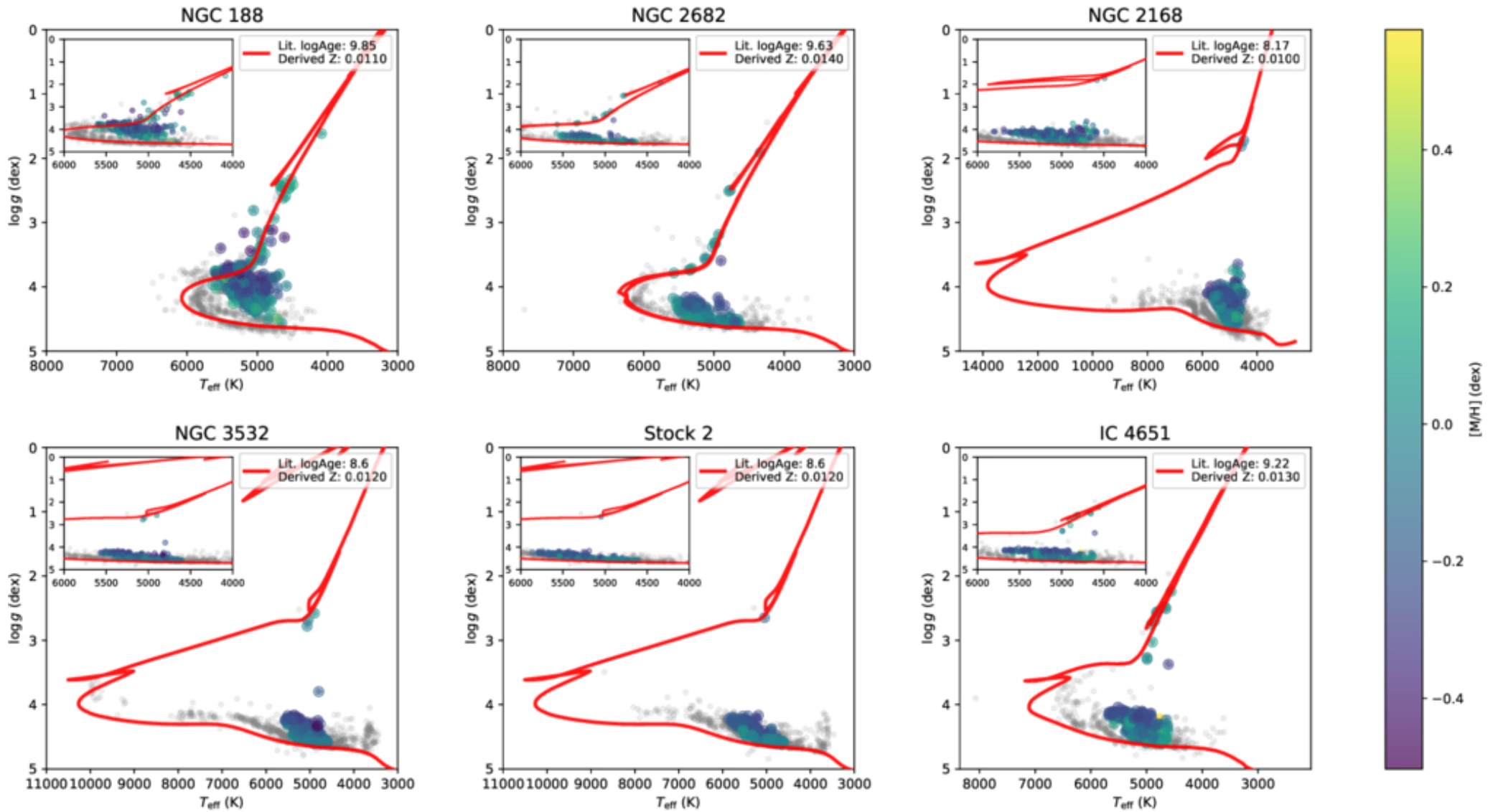
Figure 15. from Jingzhen Sun et al 2026 Astrophys. J. Suppl. 285 doi:10.3847/1538-4365/ae743e https://dx.doi.org/10.3847/1538-4365/ae743e © 2026. The Author(s). Published by the American Astronomical Society.
