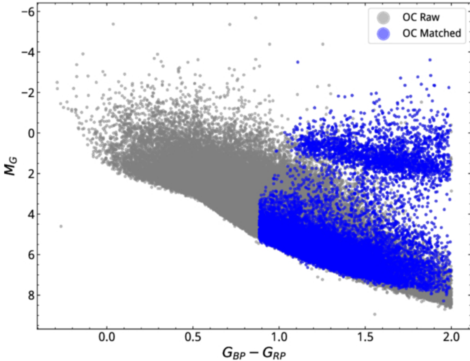
Figure 14. from Jingzhen Sun et al 2026 Astrophys. J. Suppl. 285 doi:10.3847/1538-4365/ae743e https://dx.doi.org/10.3847/1538-4365/ae743e © 2026. The Author(s). Published by the American Astronomical Society.
