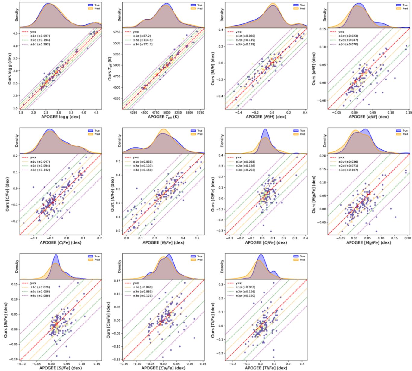
Figure 11. from Jingzhen Sun et al 2026 Astrophys. J. Suppl. 285 doi:10.3847/1538-4365/ae743e https://dx.doi.org/10.3847/1538-4365/ae743e © 2026. The Author(s). Published by the American Astronomical Society.
