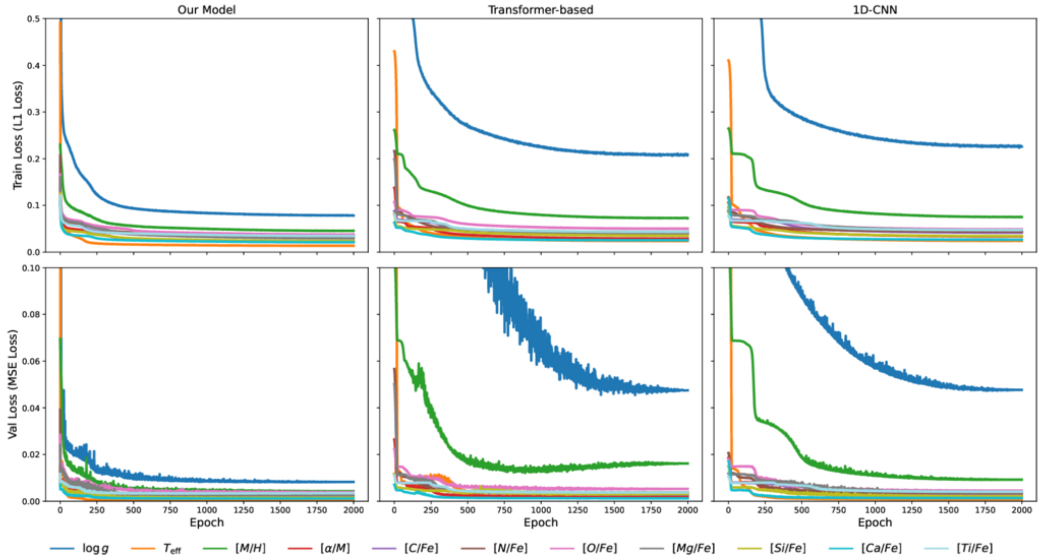
Figure 10. from Jingzhen Sun et al 2026 Astrophys. J. Suppl. 285 doi:10.3847/1538-4365/ae743e https://dx.doi.org/10.3847/1538-4365/ae743e © 2026. The Author(s). Published by the American Astronomical Society.
