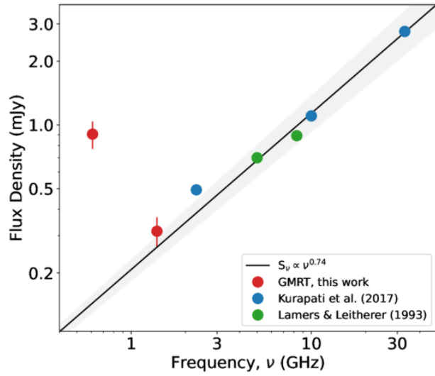
(a) HD 37742
