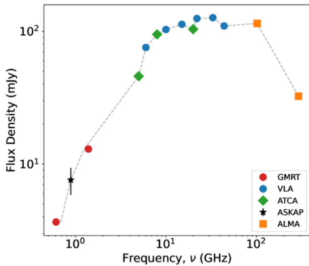
(c) HD 142184
