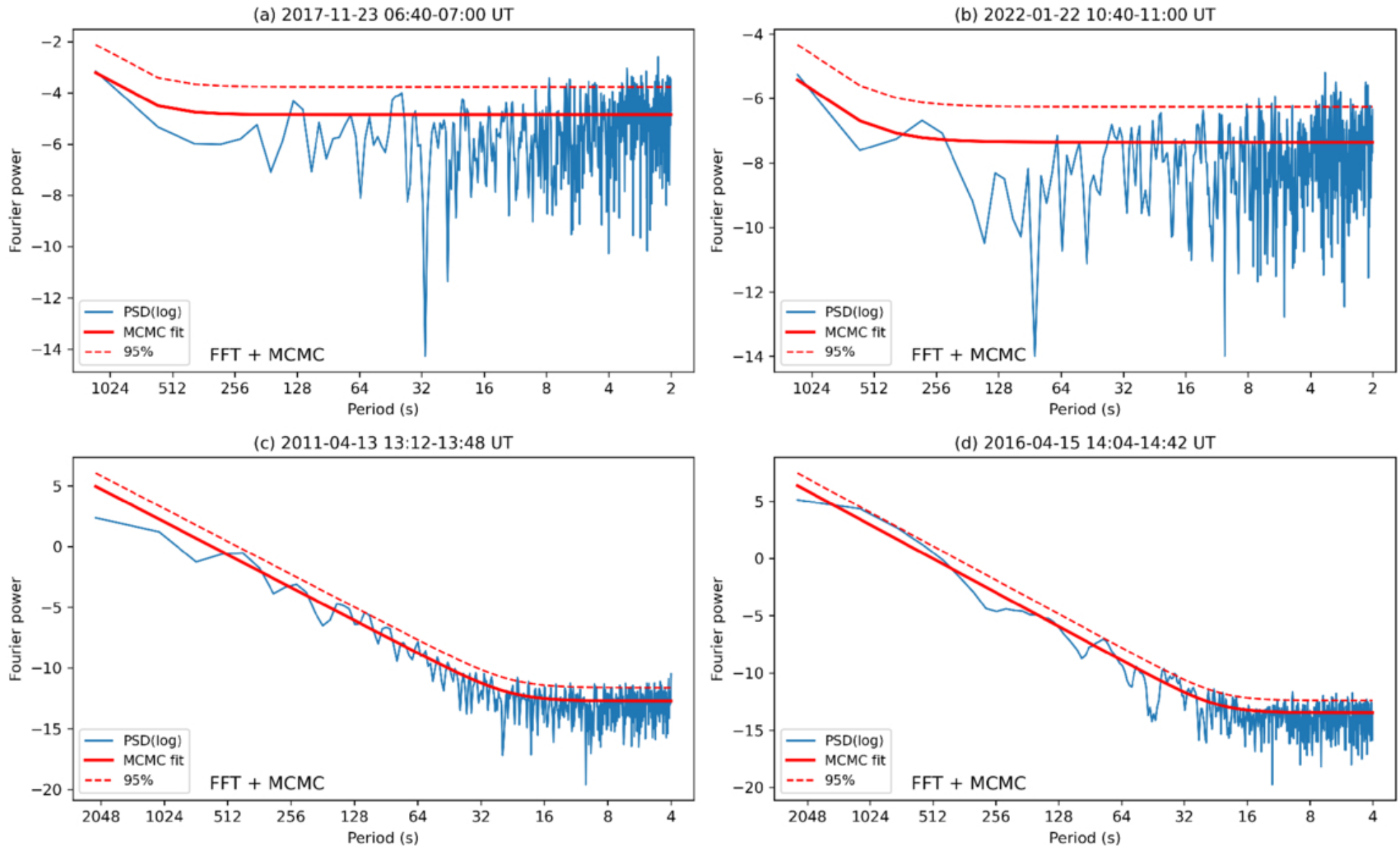
Figure 8. from Song Feng et al 2026 Astrophys. J. Suppl. 285 doi:10.3847/1538-4365/ae7345 https://dx.doi.org/10.3847/1538-4365/ae7345 © 2026. The Author(s). Published by the American Astronomical Society.
