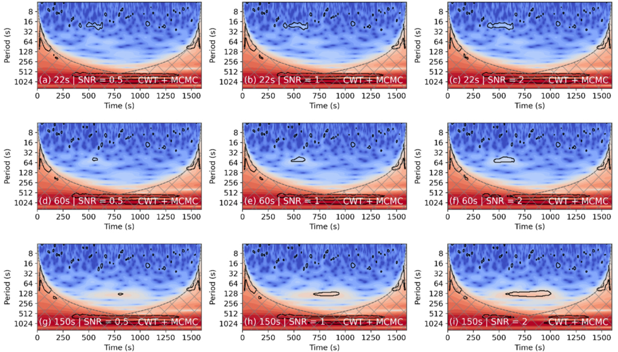
Figure 4. from Song Feng et al 2026 Astrophys. J. Suppl. 285 doi:10.3847/1538-4365/ae7345 https://dx.doi.org/10.3847/1538-4365/ae7345 © 2026. The Author(s). Published by the American Astronomical Society.
