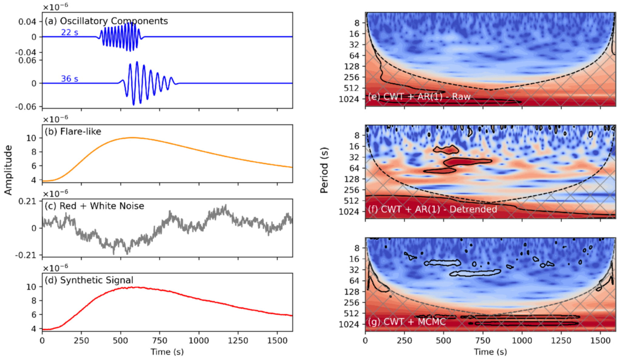
Figure 2. from Song Feng et al 2026 Astrophys. J. Suppl. 285 doi:10.3847/1538-4365/ae7345 https://dx.doi.org/10.3847/1538-4365/ae7345 © 2026. The Author(s). Published by the American Astronomical Society.
