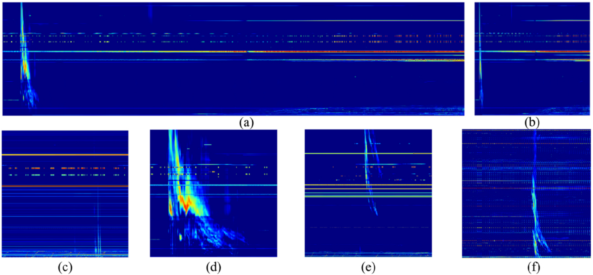
Figure 3. from Yan Liu et al 2026 Astrophys. J. Suppl. 285 doi:10.3847/1538-4365/ae7337 https://dx.doi.org/10.3847/1538-4365/ae7337 © 2026. The Author(s). Published by the American Astronomical Society.
