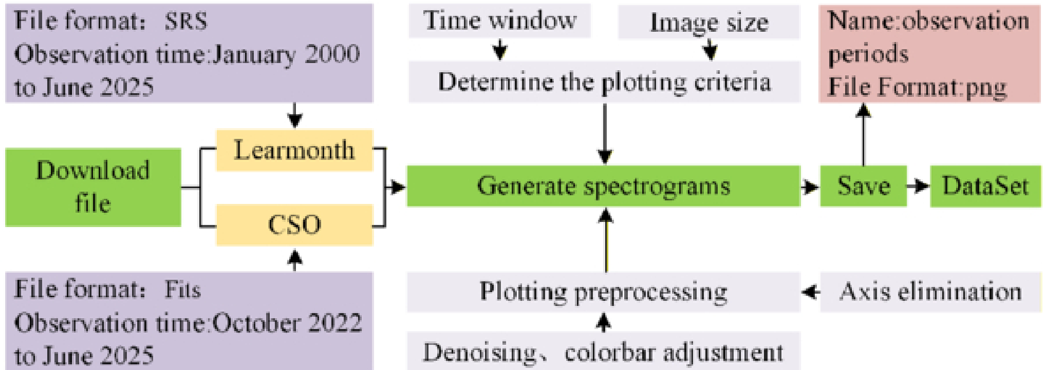
Figure 2. from Yan Liu et al 2026 Astrophys. J. Suppl. 285 doi:10.3847/1538-4365/ae7337 https://dx.doi.org/10.3847/1538-4365/ae7337 © 2026. The Author(s). Published by the American Astronomical Society.
