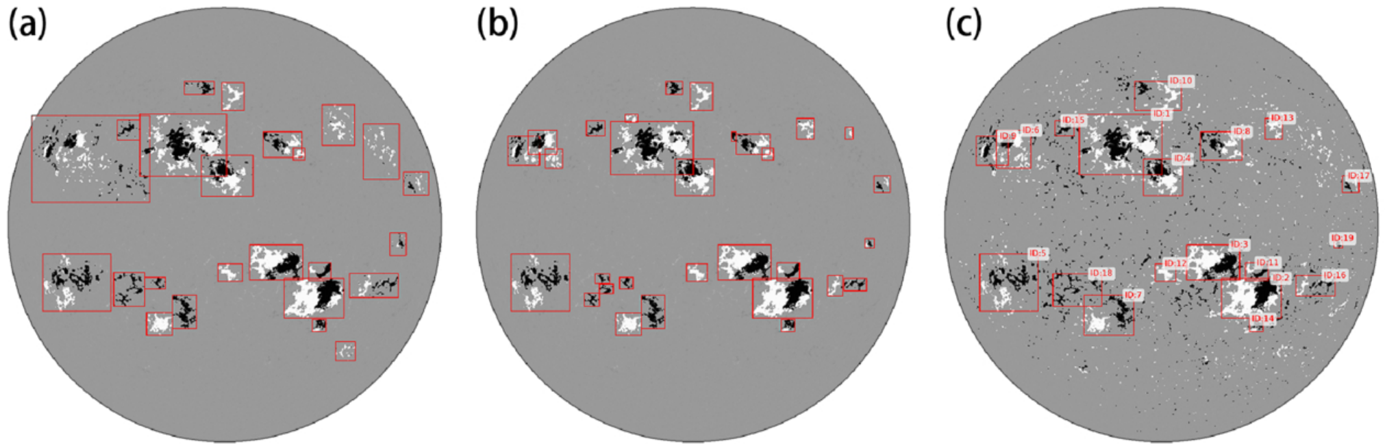
Figure 3. from C. X. Shi et al 2026 Astrophys. J. Suppl. 285 doi:10.3847/1538-4365/ae6fb3 https://dx.doi.org/10.3847/1538-4365/ae6fb3 © 2026. The Author(s). Published by the American Astronomical Society.
