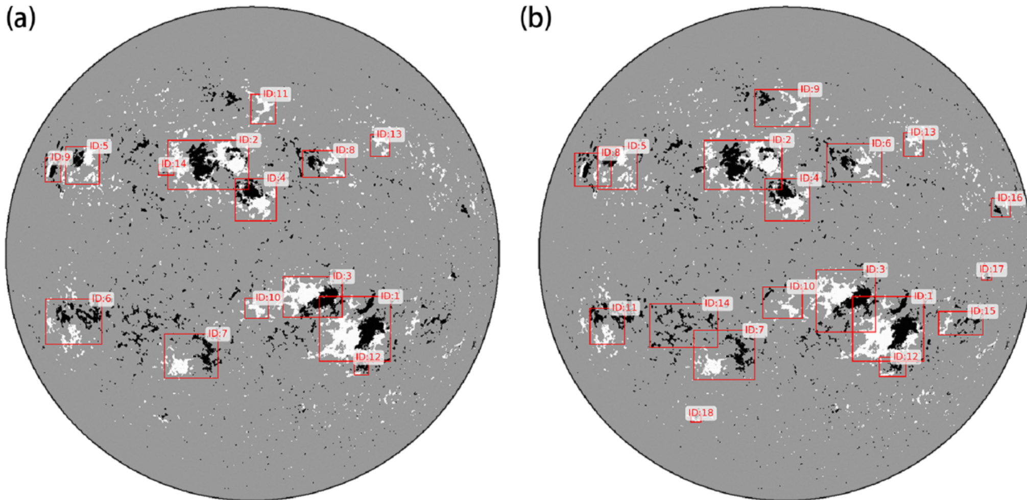
Figure 2. from C. X. Shi et al 2026 Astrophys. J. Suppl. 285 doi:10.3847/1538-4365/ae6fb3 https://dx.doi.org/10.3847/1538-4365/ae6fb3 © 2026. The Author(s). Published by the American Astronomical Society.
