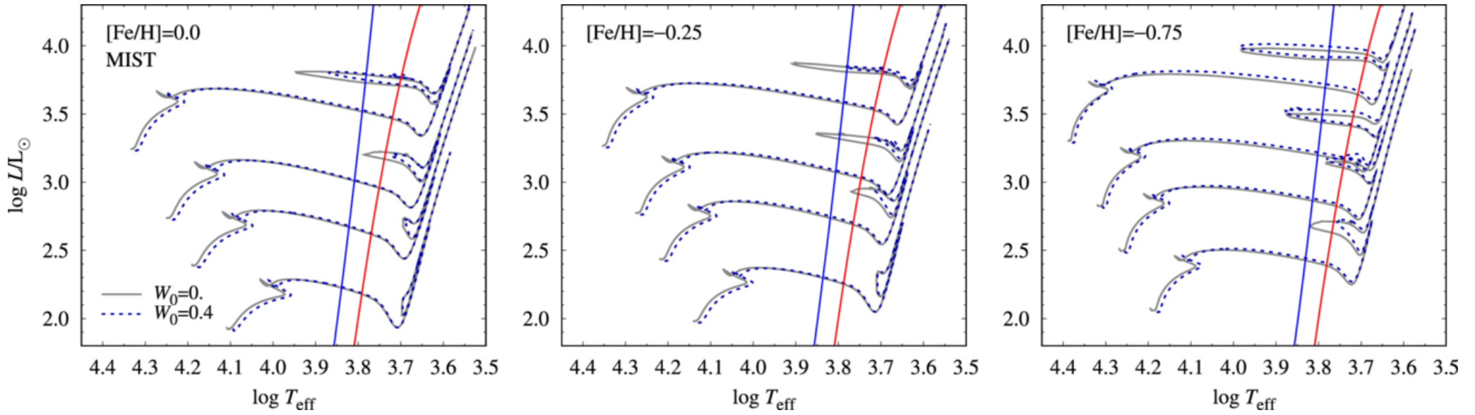
Figure 9. from Radoslaw Smolec et al 2026 Astrophys. J. Suppl. 285 doi:10.3847/1538-4365/ae6ef3 https://dx.doi.org/10.3847/1538-4365/ae6ef3 © 2026. The Author(s). Published by the American Astronomical Society.
